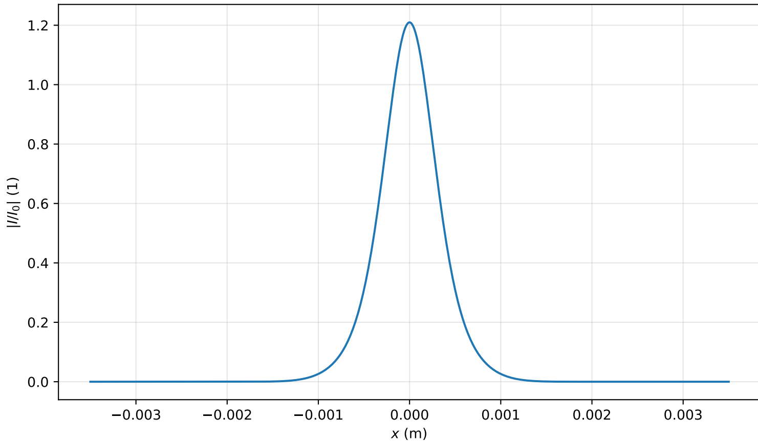
Intensity profile I(x, y = 0, z = 1.115m)/I_0 , P_{in}=0.7P_{cr} , artificial time
